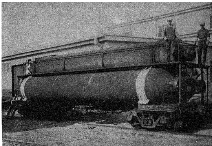
FIG. 120.—Tank car for the transportation of helium gas. Under a pressure of 2,000 lb./sq. in. in these cylinders, the gas will occupy about 200,000 cu. ft. when expanded to atmospheric pressure. ( Courtesy of U.S. Department of Commerce. )
