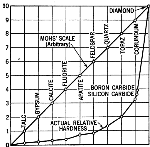
FIG. 132.—Arbitrary and actual scales of hardness.
