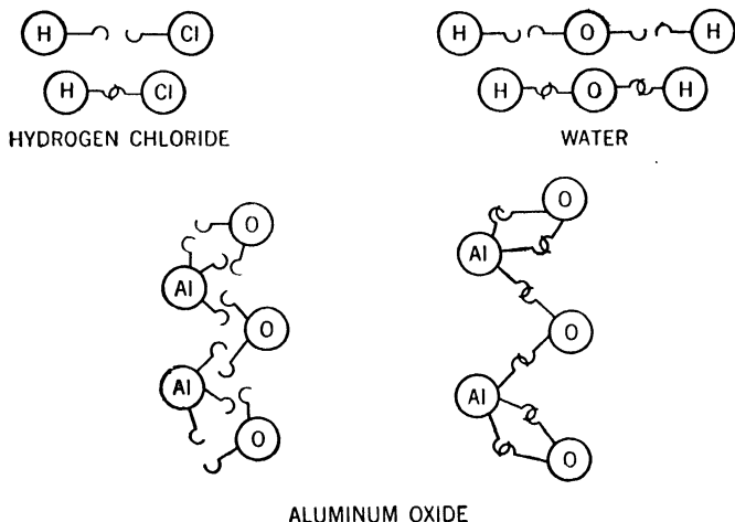
FIG. 23.—Valence bonds.
