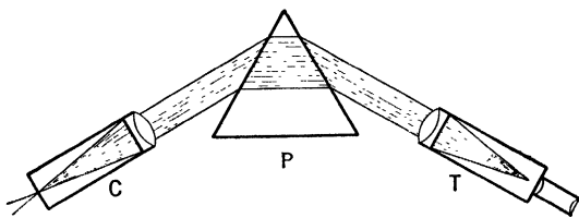
FIG. 85.—A spectroscope.
