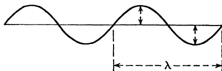
FIG. 83.—Wave-length and amplitude.
