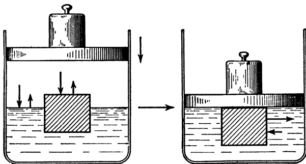
FIG. 52.—The effect of pressure on the melting point.
