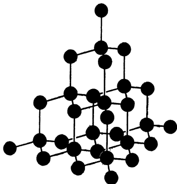
FIG. 58.—Diamond.
