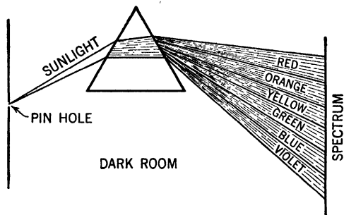
FIG. 84.—Dispersion of white light by a prism.
