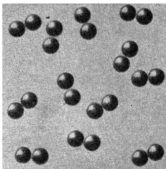
Oxygen
