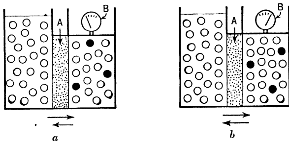
FIG. 71.—Osmotic pressure.
