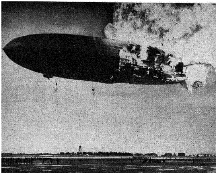
FIG. 27.—The combustion of hydrogen on a large scale. The airship Hindenburg was destroyed by fire on May 6, 1937. (Courtesy of Press Association, Inc.)
