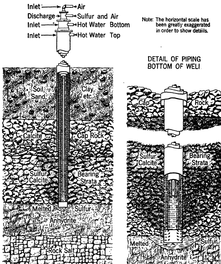
FIG. 114.—The Frasch process. (Courtesy of Texas Gulf Sulphur Company.)
