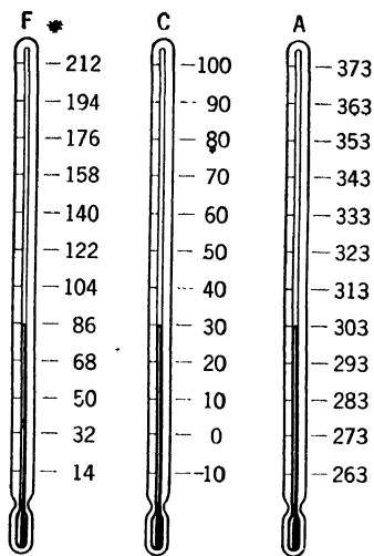
FIG. 30.—Temperature scales.
