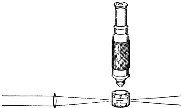
FIG. 142.—An ultramicroscope.
