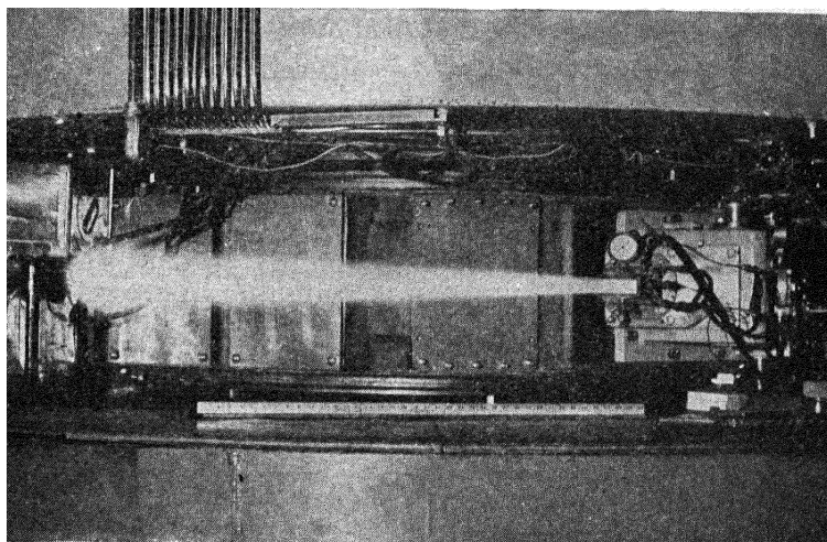
FIG. 108.—A beam of purple light marks the path of a stream of deuterons emerging from the cyclotron. (Courtesy of Dr. Donald Cooksey and the Radiation Laboratory at the University of California.)
