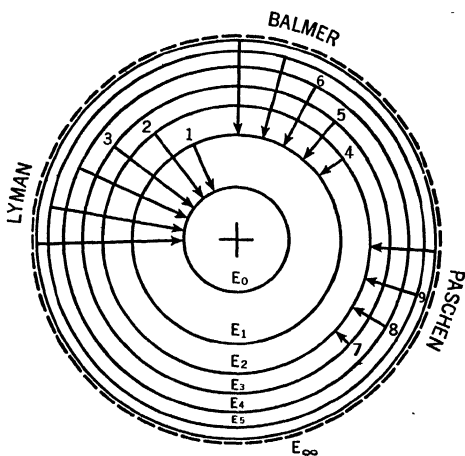
FIG. 88.—Energy levels in the hydrogen atom.
