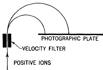
FIG. 106.—Mass spectrograph.
